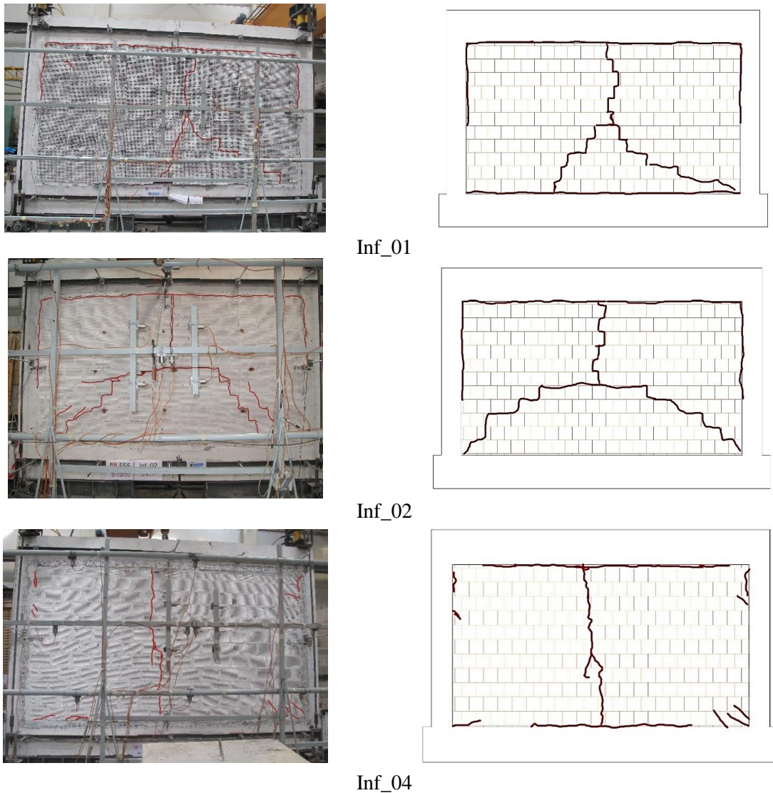
Figure 2. Test results: Damages observed and cracking pattern.
